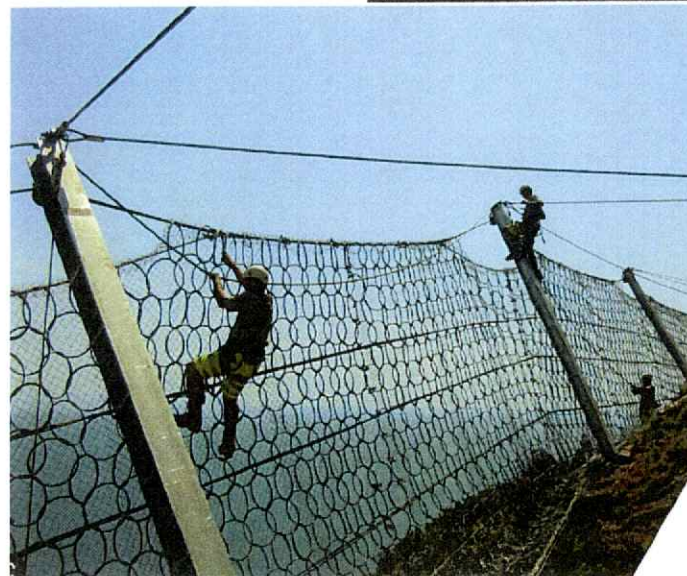
Rock mitigation fence
